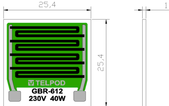
Fig. 1. Preview with dimensions [mm]
